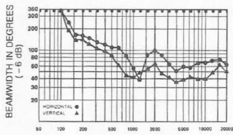
FIGURE 3 FS-212A Beamwidth vs. Frequency
